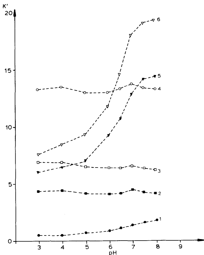
Fig. 3. Influence of the pH of the mobile phase on the capacity ratios ( k' ) of amphetamine and impurities. 1 = Amphetamine; 2 = N-formylamphetamine; 3 = 4-methyl-5-phenylpyrimidine; 4 = N,N-di( \beta -phenylisopropyl)formamide; 5 = N,N-di( \beta -phenylisopropyl)amine; 6 = N,N-di( \beta -phenylisopropyl)methylamine.
